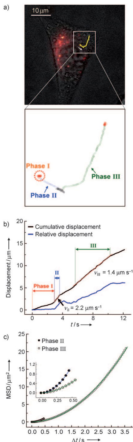
Figure 4. a) Trajectory of a vesicle containing UCNP's transported from the perinuclear region to the cell periphery presumably by kinesins. In phase I, the vesicle is initially confined in a small area. The segments of the trajectory, which display approximately linear paths, are designated as phases II and III. b) Cumulative and relative displacement traces for the trajectory shown in (a). The transport speeds were calculated for phases II and III by linear regression. c) MSD plots for phases II and III. They are well fit to the equation \text{MSD} = 4D\Delta t + v^2\Delta t^2 , which is indicative of active transport in two dimensions. The diffusion coefficients ( D ) were estimated to be 0.008 , 0.024 \mu\text{m}^2 \text{s}^{-1} for phases II and III, respectively.
